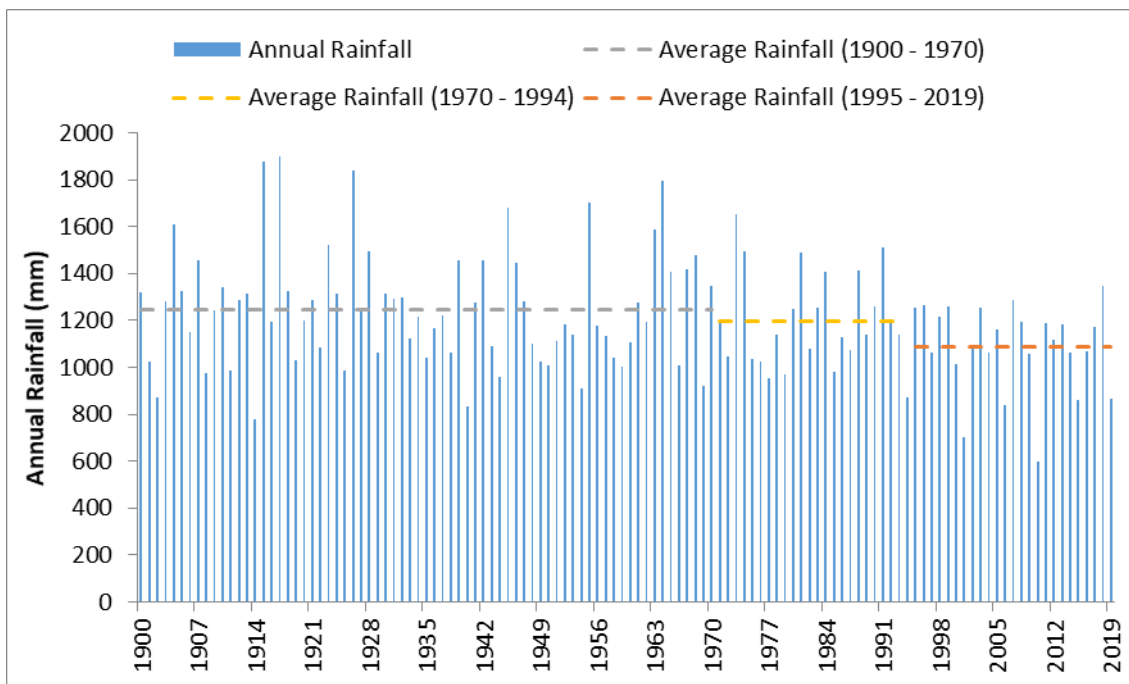
Figure 4-2 Annual rainfall at Karnet Station
