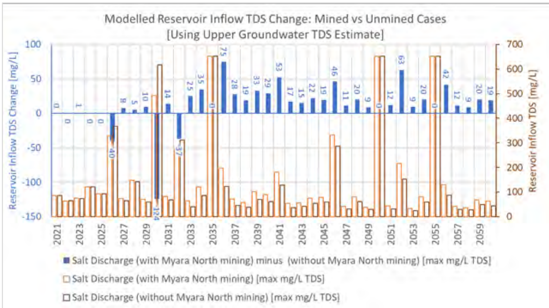
Figure 8-17 Modelled reservoir inflow TDS change, Serpentine Reservoir
