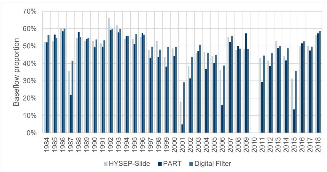
Figure 5-9 Baseflow trends
