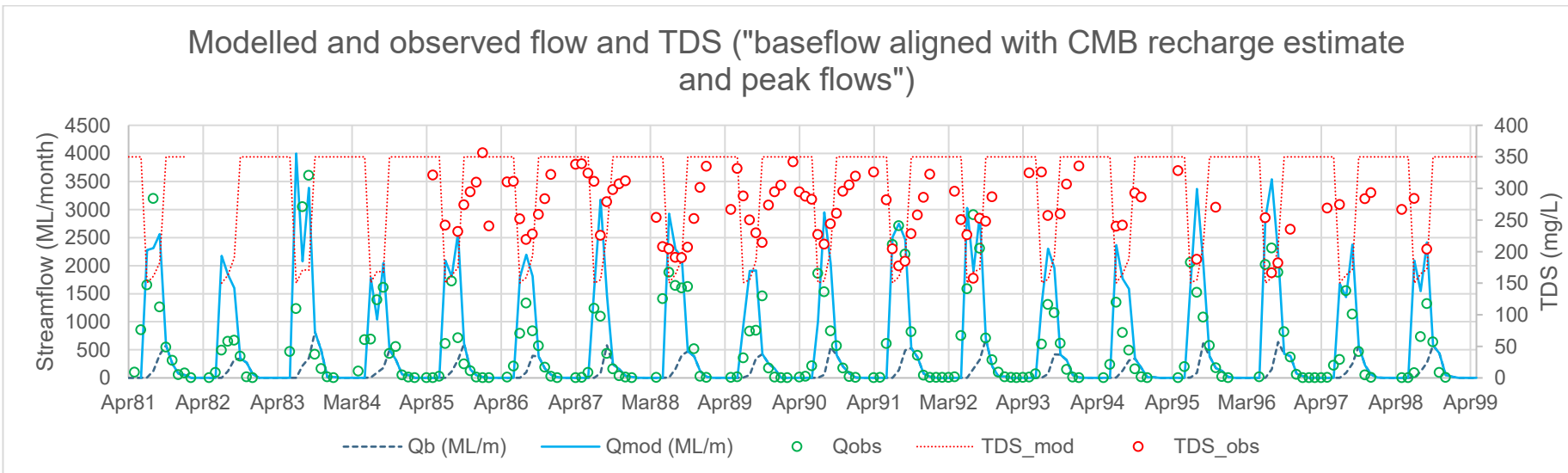
Figure 5-13 Application of simple analytical TDS-constrained baseflow-quickflow models to represent measured streamflows at Jack Rocks gauge (Qb – baseflow; Qmod – modelled streamflow; Qobs – observed streamflow; TDS_mod – modelled TDS; TDS_obs observed TDS)
