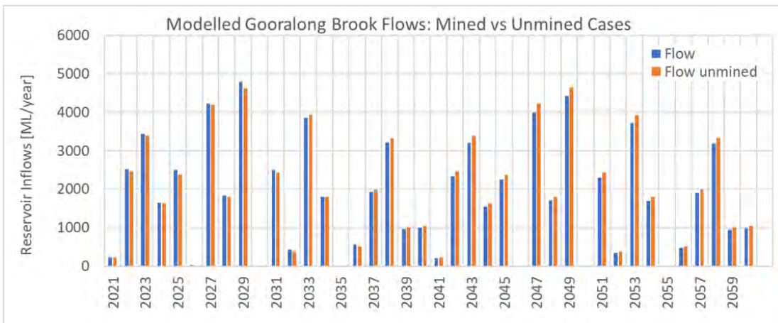
Figure 8-9 Modelled streamflow, Gooralong Brook (mined vs unmined)
